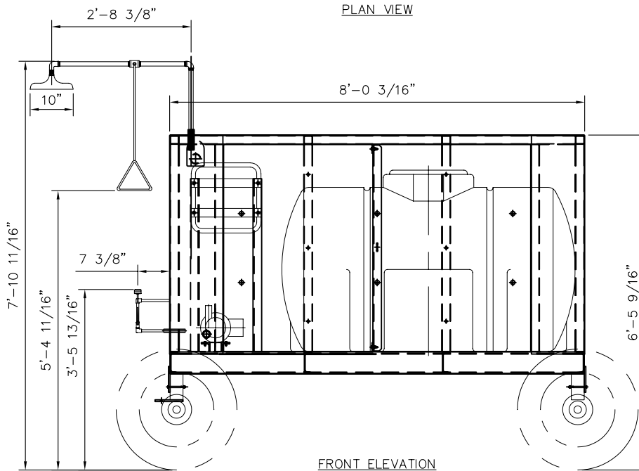
FRONT ELEVATION
