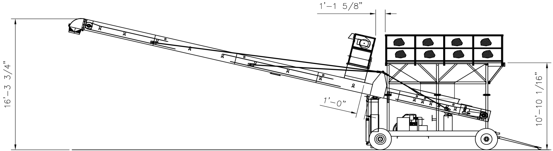
CONVEYOR WITH CYLINDER EXTENDED
